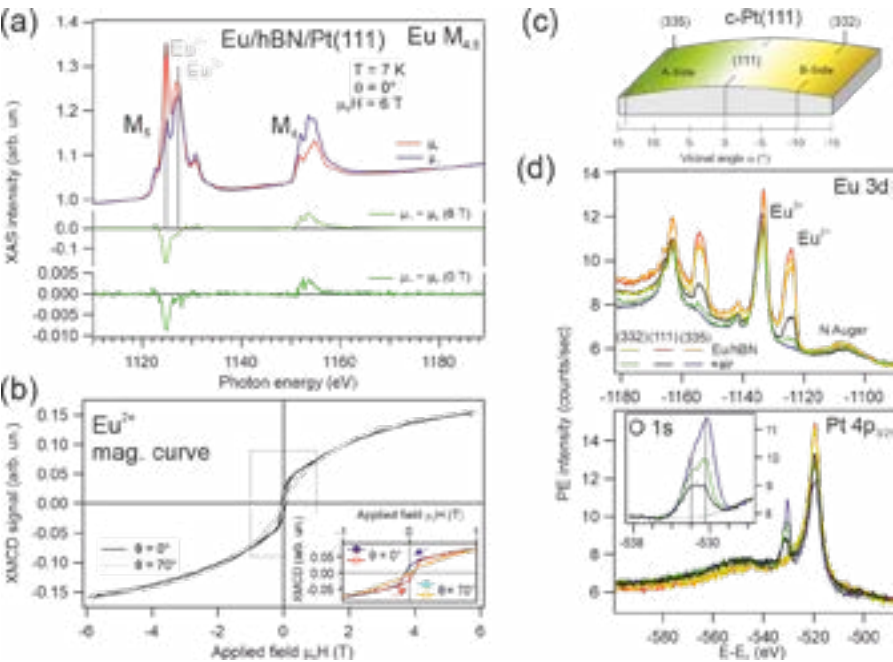
Figure 2: Magnetic and electronic properties of EuPt 2 surface compound protected by hBN. (a), (b) X-ray absorption and X-ray magnetic dichroism spectra and magnetization curves at the Eu M_{4,5} absorption edge confirming the ferromagnetic state of Eu. (c) Schematic description of the curved substrate. (d) X-ray photoemission spectroscopy prior and after air exposure of the hBN/EuPt 2 system, revealing partial chemical protection at (111) and (335) surfaces.
