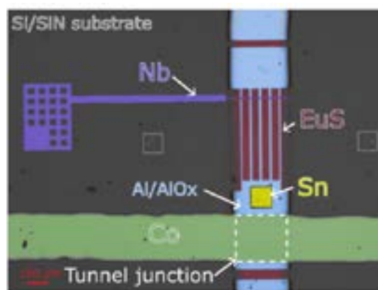
Figure 2: Fake-color optical micrograph of a SFTED calorimeter, in which the material compositions are illustrated with different colors. A superconductor-ferromagnet hetero-junction area is marked with the white dashed line, consisting of layers of Si/SiN/EuS/Al/AlOx/Co from the bottom to the top. A Sn absorber is placed to the side of the junction, contacting directly the Al lead with AlOx layer removed via chemical etching.
